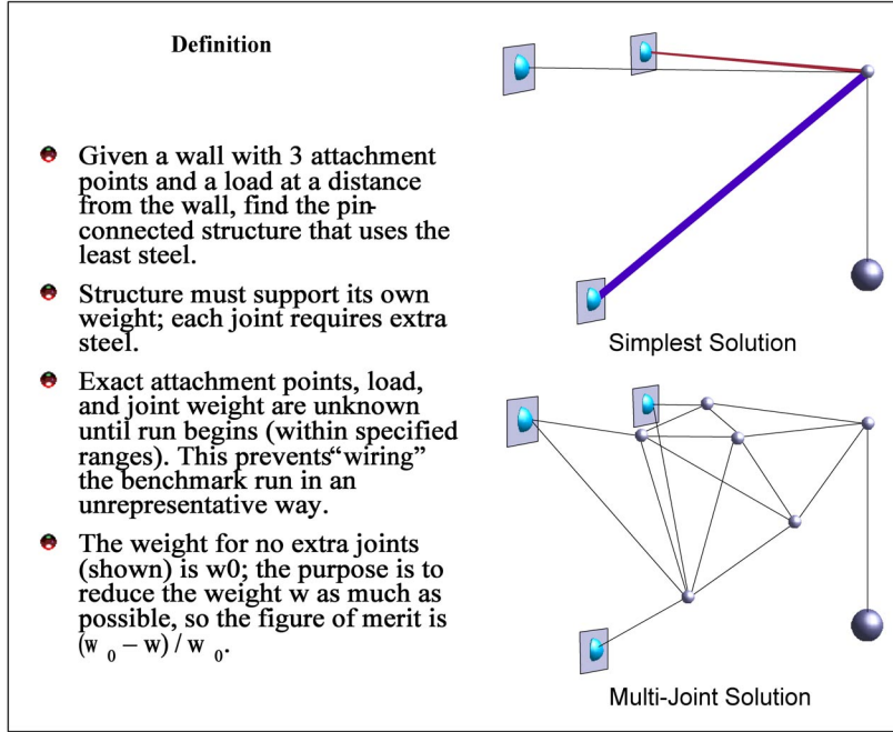
Figure 1: Truss Benchmark
