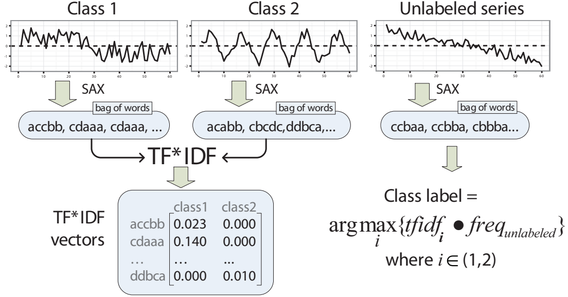
Figure 3.3: An overview of the SAX-VSM algorithm: at first, labeled time series are converted into bags of words using SAX; secondly, tf * idf statistics is computed resulting in a single weight vector per training class. For the classification, an unlabeled time series is converted into the term frequency vector and assigned a label of the weight vector that yields a maximal cosine similarity value. This is ltc.nnn weighting schema in SMART notation (Table 3.3).
