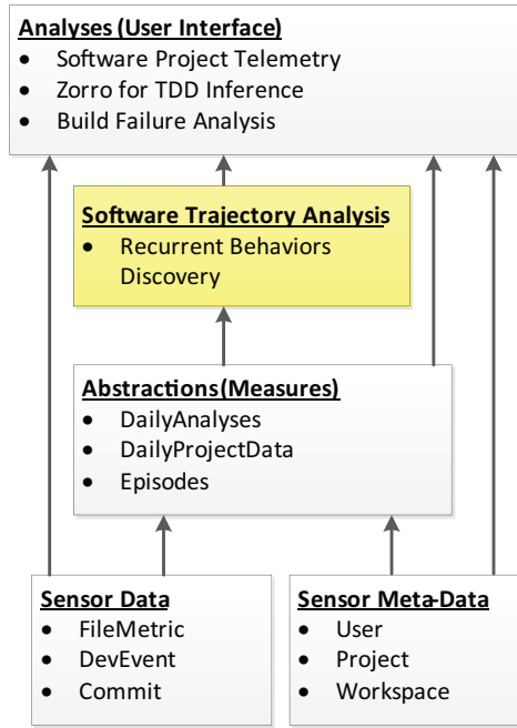
Figure 4.1: A schematic overview of the very first and the latest STA implementations. Note the STA evolution from a thin layer embedded into the larger system relying on external data assimilation and processing mechanisms to an end-to-end generic solution for software artifact measurements analysis.
