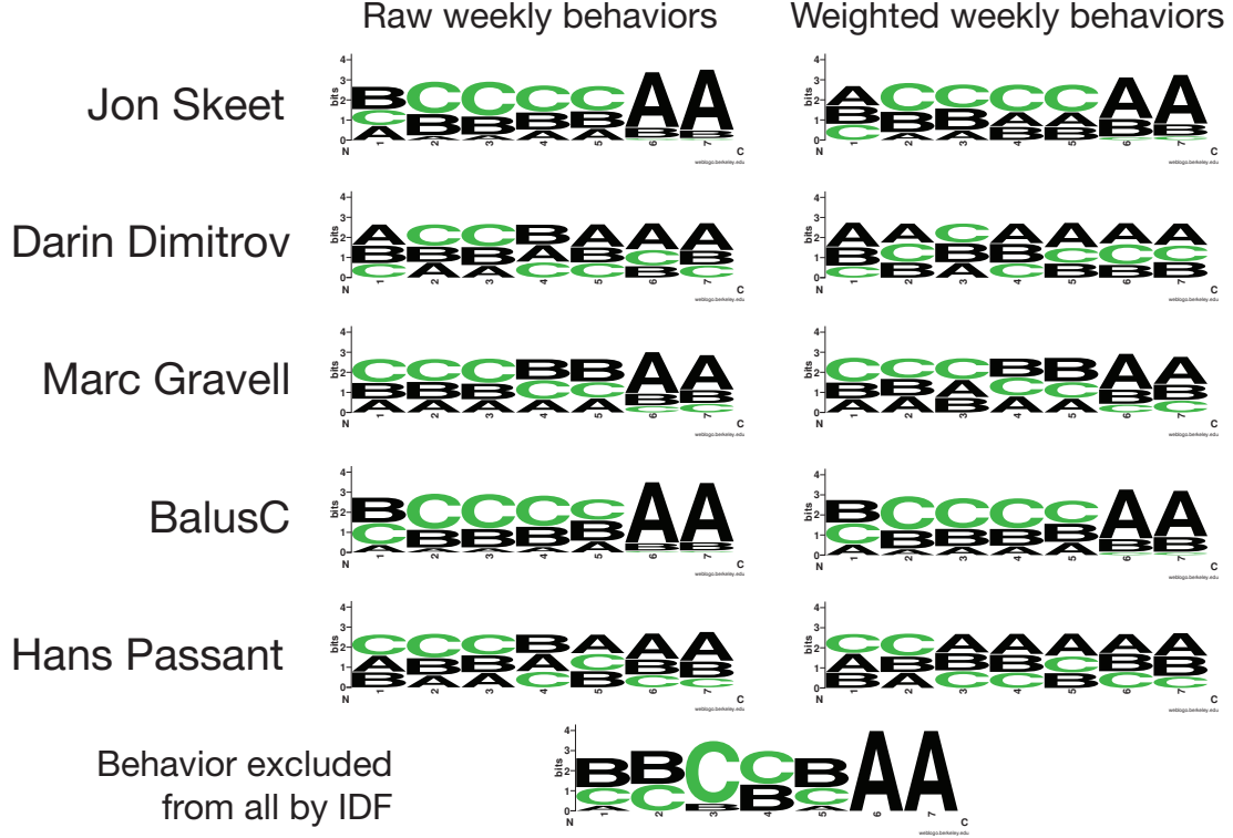
Figure 4.13: WebLogo visualization of weekly activity for top SO users. Here, letters (A,B,C) corresponds to ( low,medium , and high ) levels of activity. Note, that SAX-VSM pattern ranking process changed the effort distribution. The excluded behaviors are likely to represent a very common behavioral pattern: peaking at the mid-week performance and work-free weekends.
