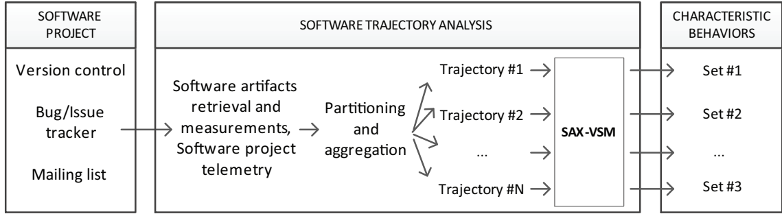
Figure 1.2: The Software Trajectory Analysis design overview. At first, software measurements are acquired directly from an external measurement engine such as Hackstat, or/and by collecting and measuring of software artifacts. Next, the measurements are used by an expert for construction of a set of software trajectories that potentially can shed light on a research question. Finally, recurrent characteristic patterns are discovered and weighted by class importance with SAX-VSM.
