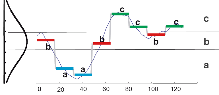
Figure 3.2: An illustration of the SAX approach taken from [4] depicts two pre-determined break-points for the three-symbols alphabet and the conversion of the time series of length n = 128 into PAA representation followed by mapping of the PAA coefficients into SAX symbols with w = 8 and a = 3 resulting in the string “ baabccbc ”.
