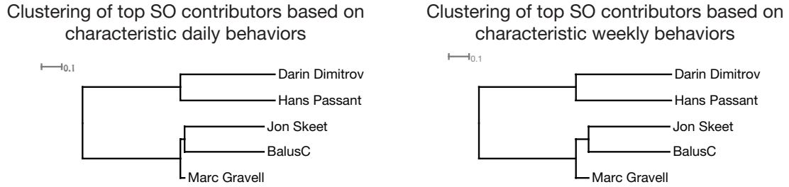
Figure 4.14: Clustering of StackOverflow user behaviors with STA. Note that D.Dimitrov’s characteristic behaviors were found very different from those of J. Skeet, while their overall reputation scores are next to each other.
