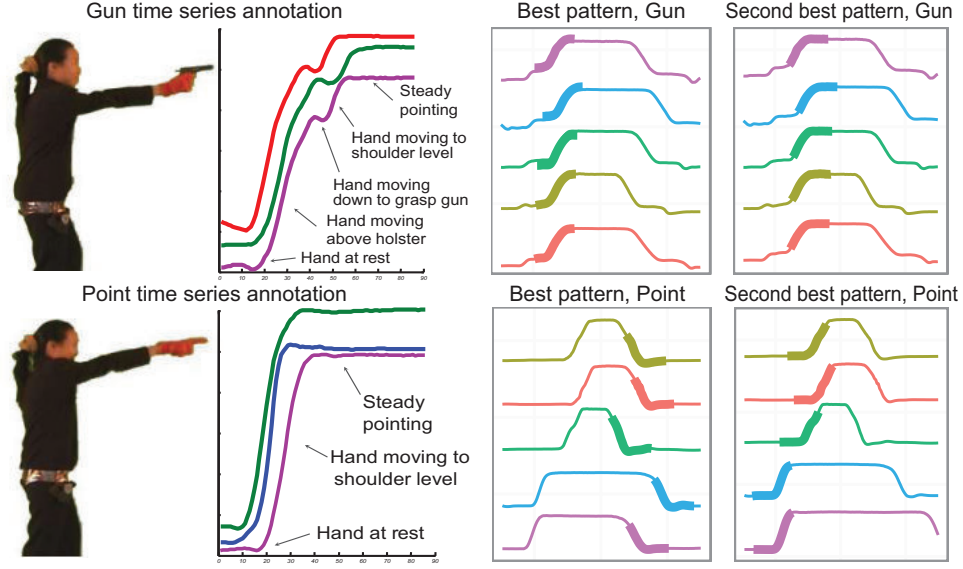
Figure 3.15: Best class-characteristic subsequences (right panels, bold lines) discovered by SAX-VSM in the Gun/Point data set. Left panels show actor’s stills and the time series annotation made by an expert while the right panels show locations of characteristic subsequences. Note, that while the upward arm motion found to be more “important” in the Gun class (gun retrieval and aiming), the downward arm motion better characterizes the Point class (note the “overshoot” phenomena in proplless arm return). This result aligns with previous work [88] and [161]. (Stills and annotation are used with a permission from E. Keogh)
