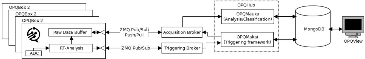
Fig. 1. OPQ System Architecture
