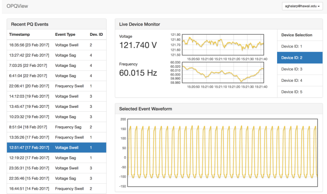
Fig. 4. OPQView Realtime Measurements and PQ Events
